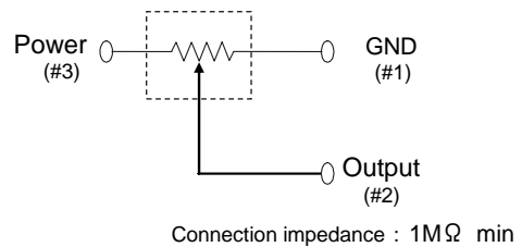
Fig.3 Circuit Diagram
