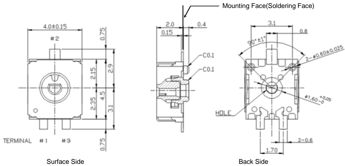
Fig.1 Dimensions
