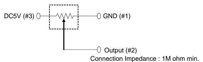
Fig.6 Circuit Diagram
