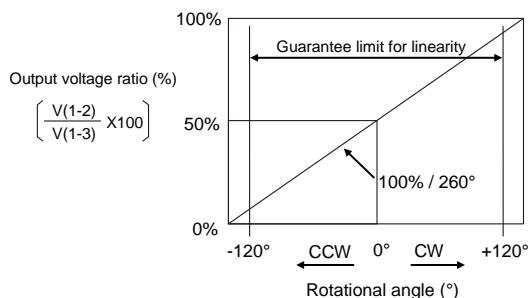
Fig.5 Linearity
