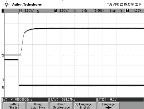
On/Off Enable Delay (Vin=48V, Vout=nom., Iout=10A, Cload=5000uF, Ta=+25° C., ScopeBW=20Mhz, Trace 2=Vout, Trace 4=Enable.
