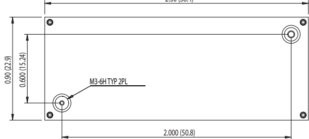
WITH BASEPLATE OPTION (Baseplate not available for UEE-3.3/15-D48 models.)
