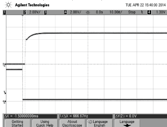
On/Off Enable Delay (Vin=48V, Vout=nom., Iout=0, Cload=0, Ta=+25° C., ScopeBW=20Mhz, Trace 2=Vout, Trace 4=Enable.
