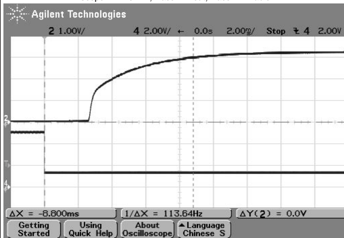
On/Off Enable Delay (Vin=48V, Vout=nom., Iout=30A, Cload=10uF, Ta=+25° C., ScopeBW=20Mhz, Trace 2=Vout, Trace 4=Enable).
