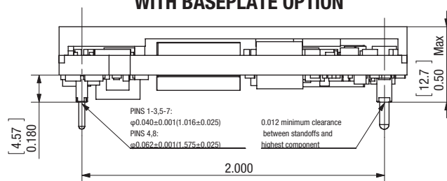
WITH BASEPLATE OPTION
