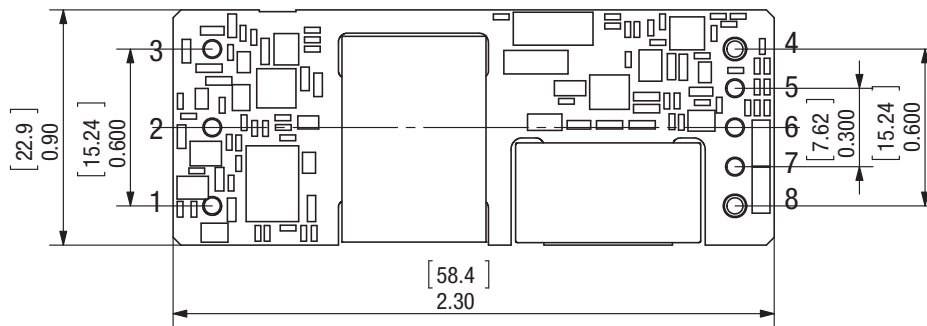
PIN SIDE VIEW
