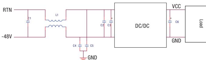
Figure 2. Conducted Emissions Test Circuit
