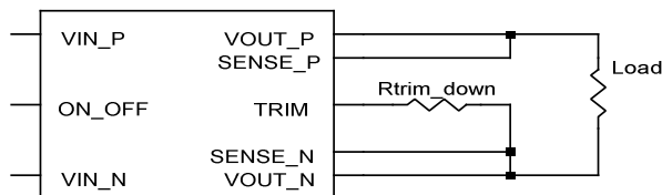
Figure 5. Trim Down connections to decrease Vout
