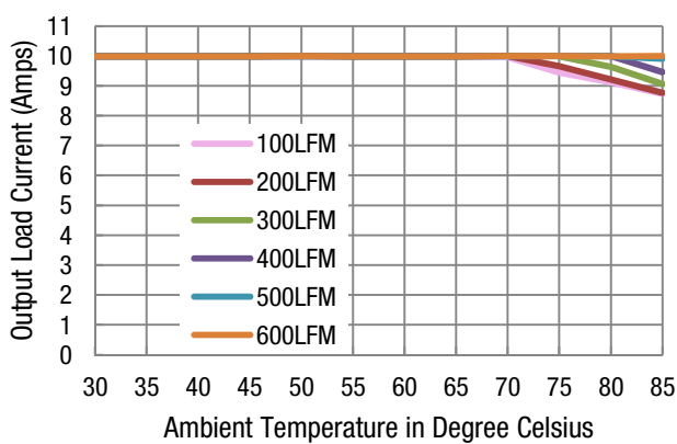
Maximum Current Temperature Derating (Open Frame) (Vin = 12V airflow is from Vin- to Vin+)
