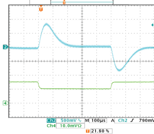
Stepload Transient Response (Vin=48V, Iout=50-75-50% of Imax, Cload=1µF || 10µF, Io=10A/div, Ta=+25°C) Ch2=Vout, Ch4=Iout
