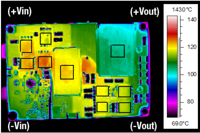
Thermal image with hot spot at 10.8A with 25°C ambient temperature. Natural convection is used with no forced airflow. Identifiable and recommended maximum value to be verified in application.
