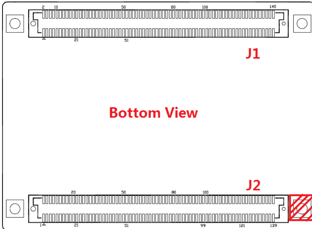
Figure 1-8 Expansion Connectors of MYC-C7Z010/20
