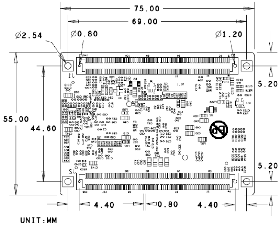
Figure 1-7 Dimensions of MYC-C7Z010/20
