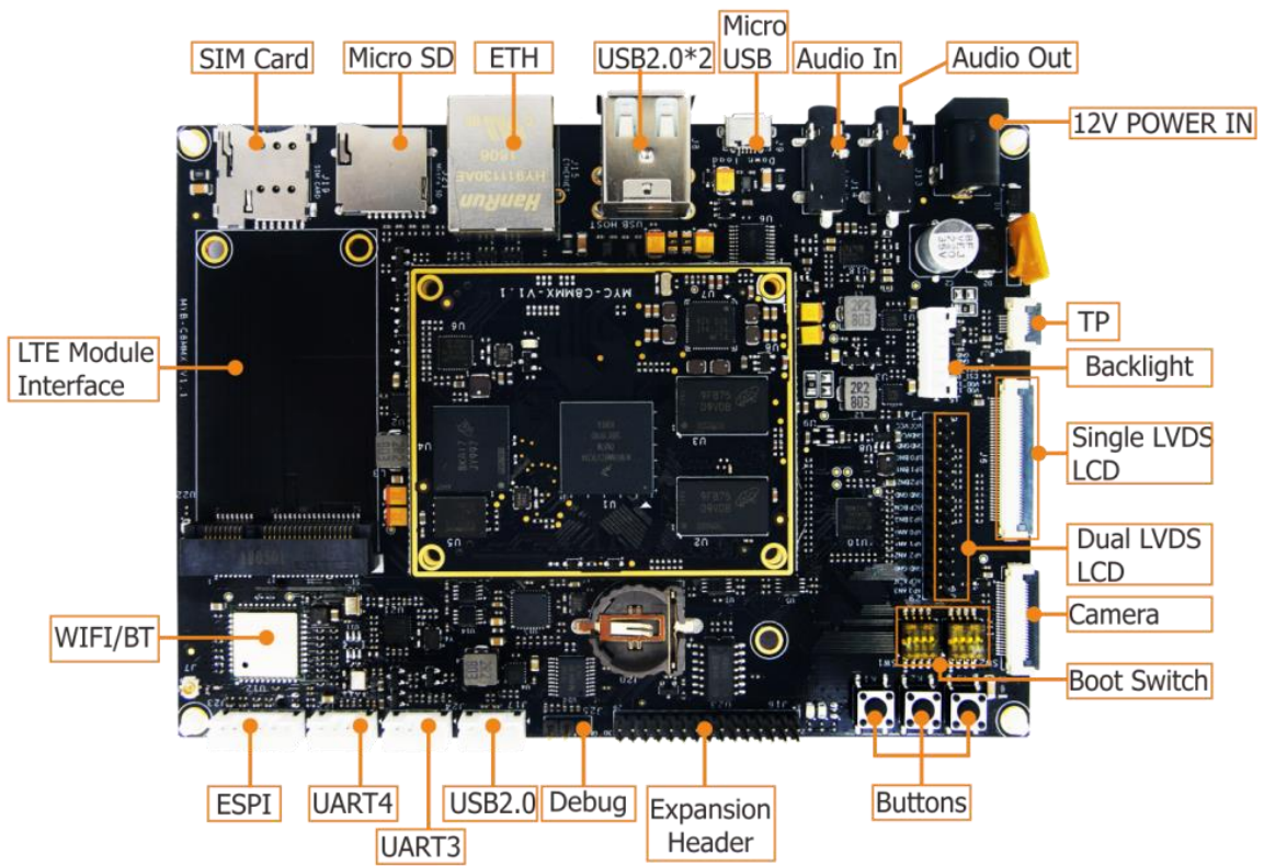
Figure 1-4 MYD-C8MMX Development Board
