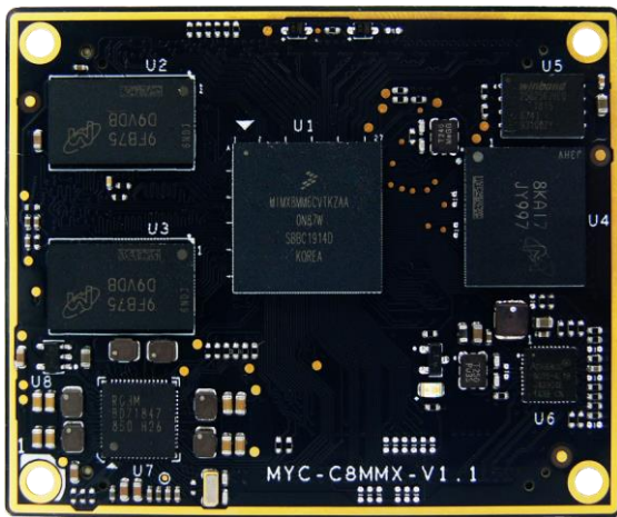
Figure 1-1 MYC-C8MMX CPU Module Top-View
