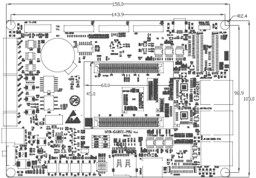
Figure 1-11 Dimension Chart of MYD-C437X-PRU
