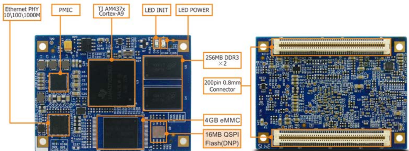
Figure 1-6 MYC-C437X CPU Module
