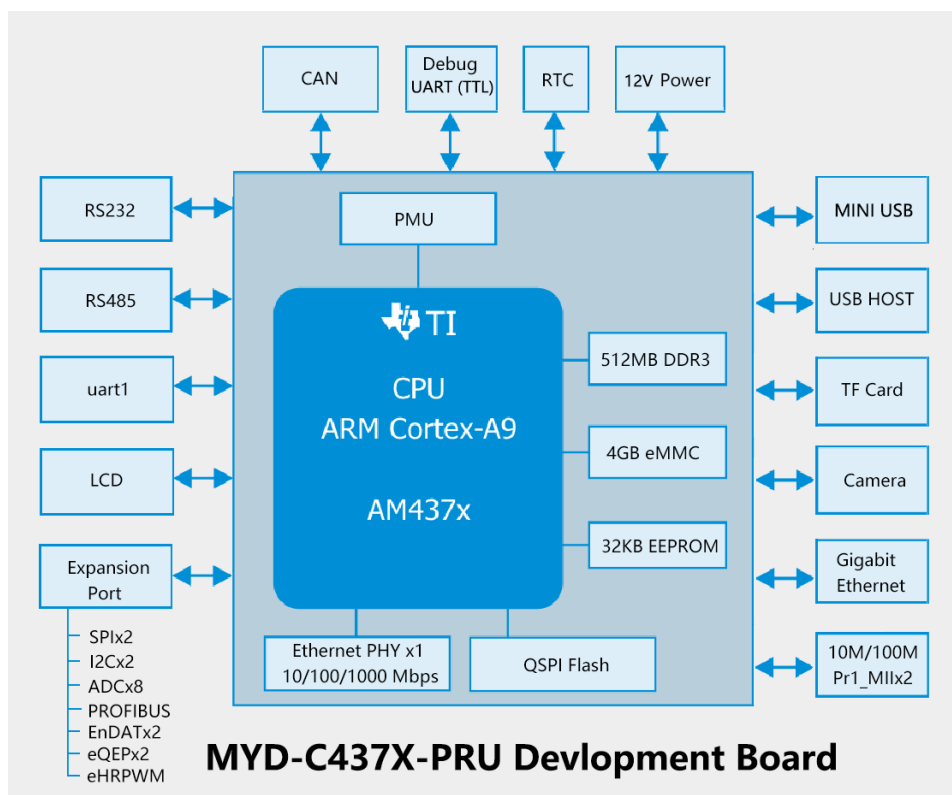
Figure 1-9 Function Block Diagram of MYD-C437X-PRU
