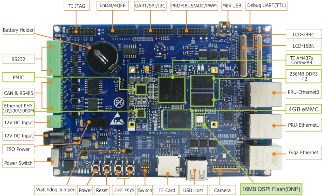
Figure 1-2 MYD-C437X-PRU Development Board
