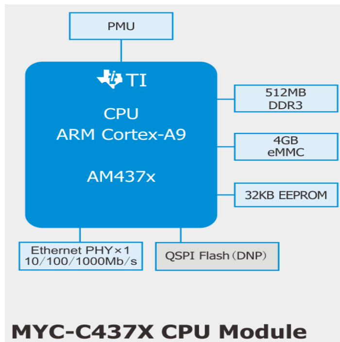
Figure 1-8 MYC-C437X Function Block Diagram
