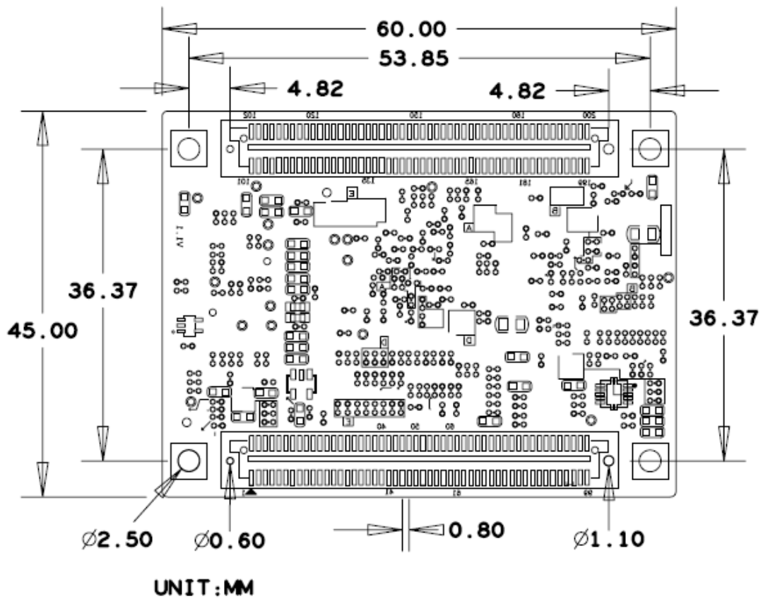
Figure 1-10 Dimension Chart of MYC-C437X CPU Module
