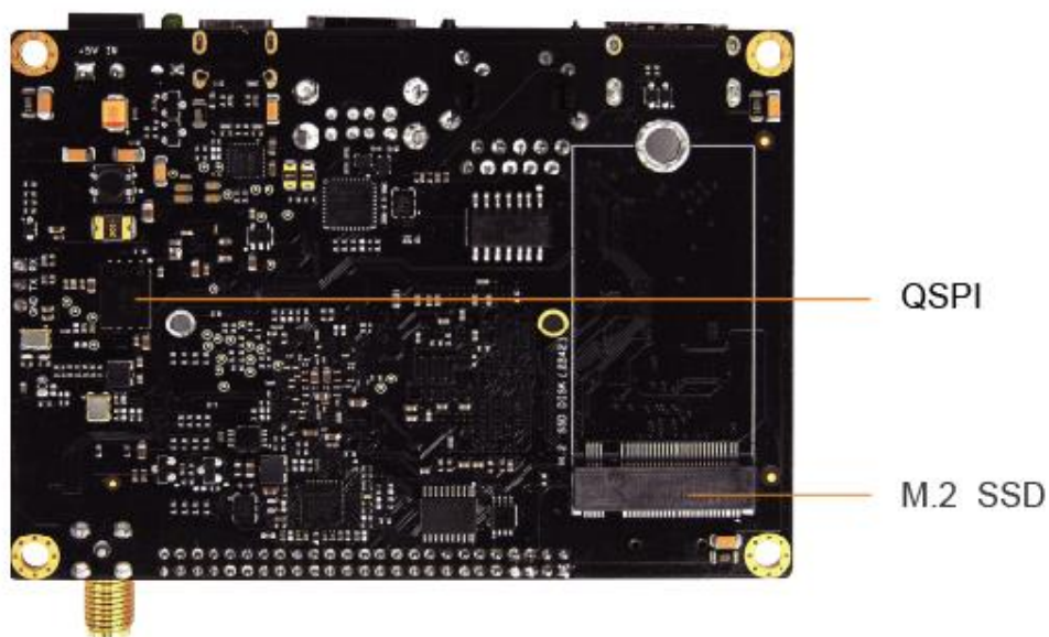
Figure 1-3 MYS-8MMX Board Bottom-View
