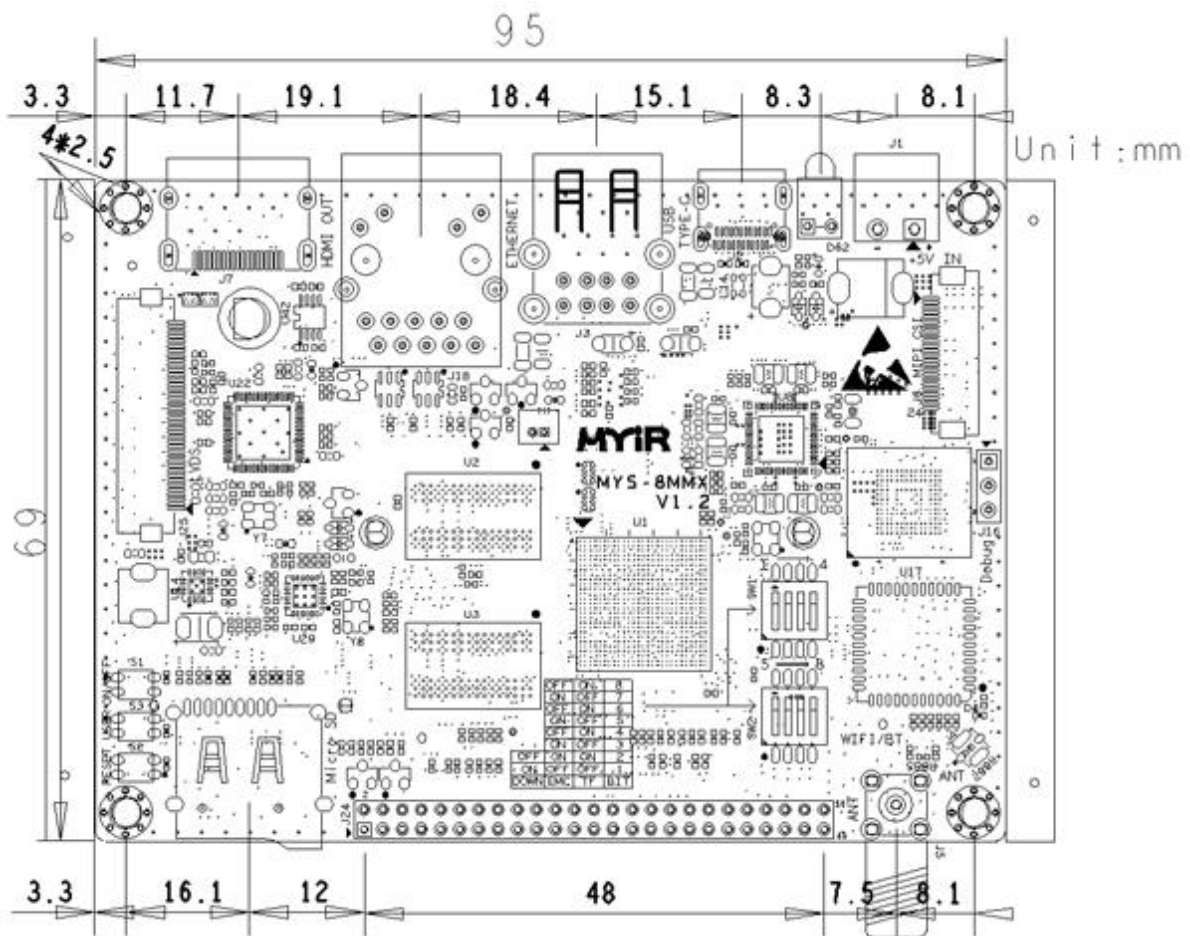
Figure 1-8 MYS-8MMX Single Board Computer Dimensions Chart
