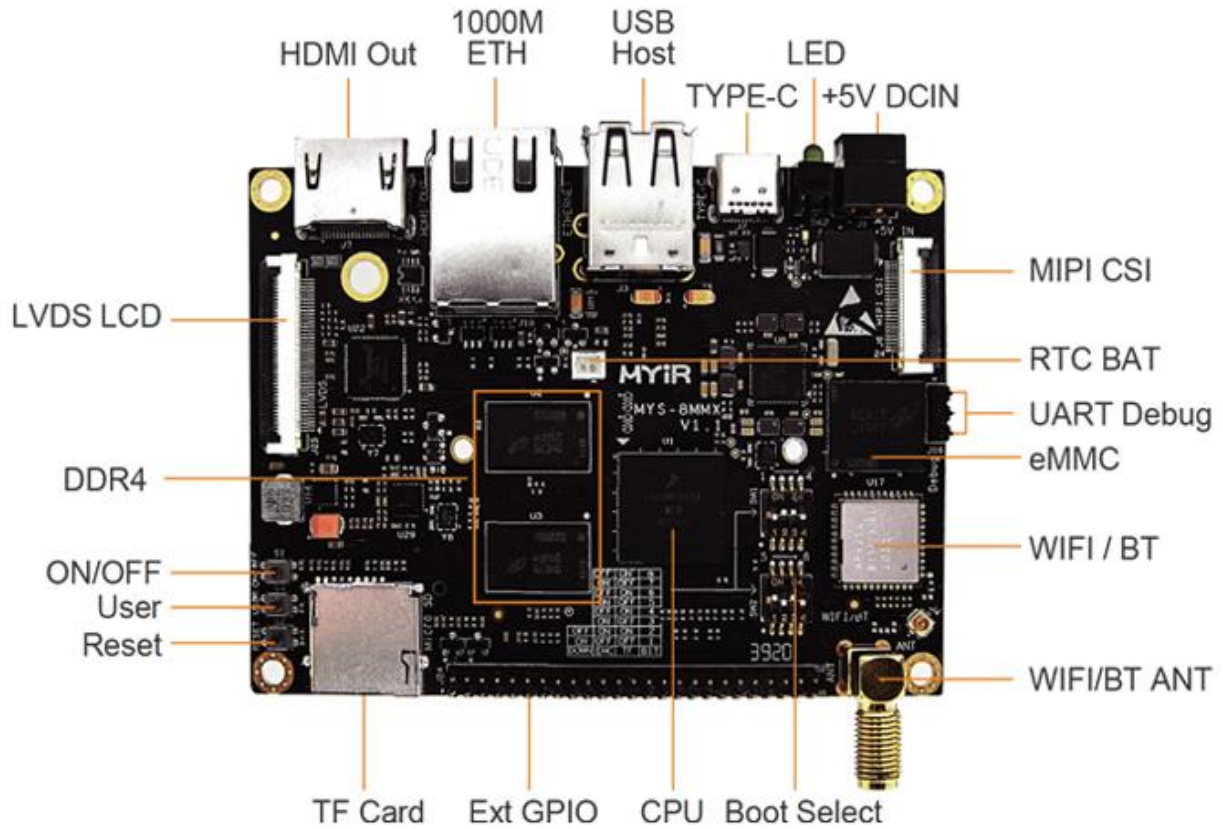
Figure 1-2 MYS-8MMX Top-View
