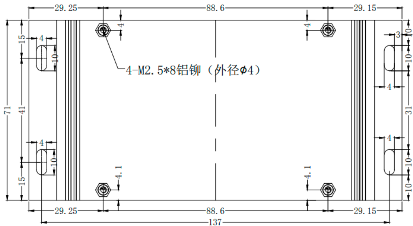
Figure 1-9 MYS-8MMX Box Dimensions Chart (Top-view)
