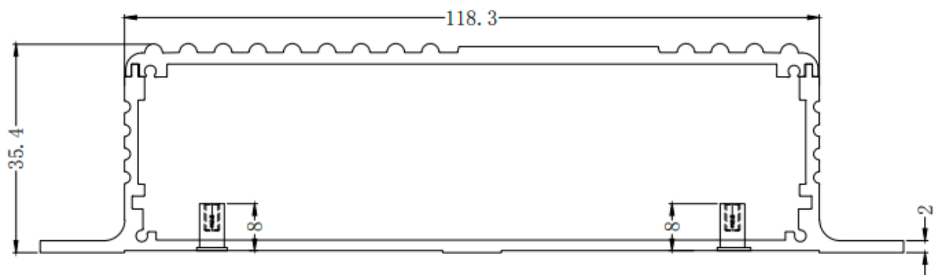
Figure 1-10 MYS-8MMX Box Dimensions Chart (Front-view)
