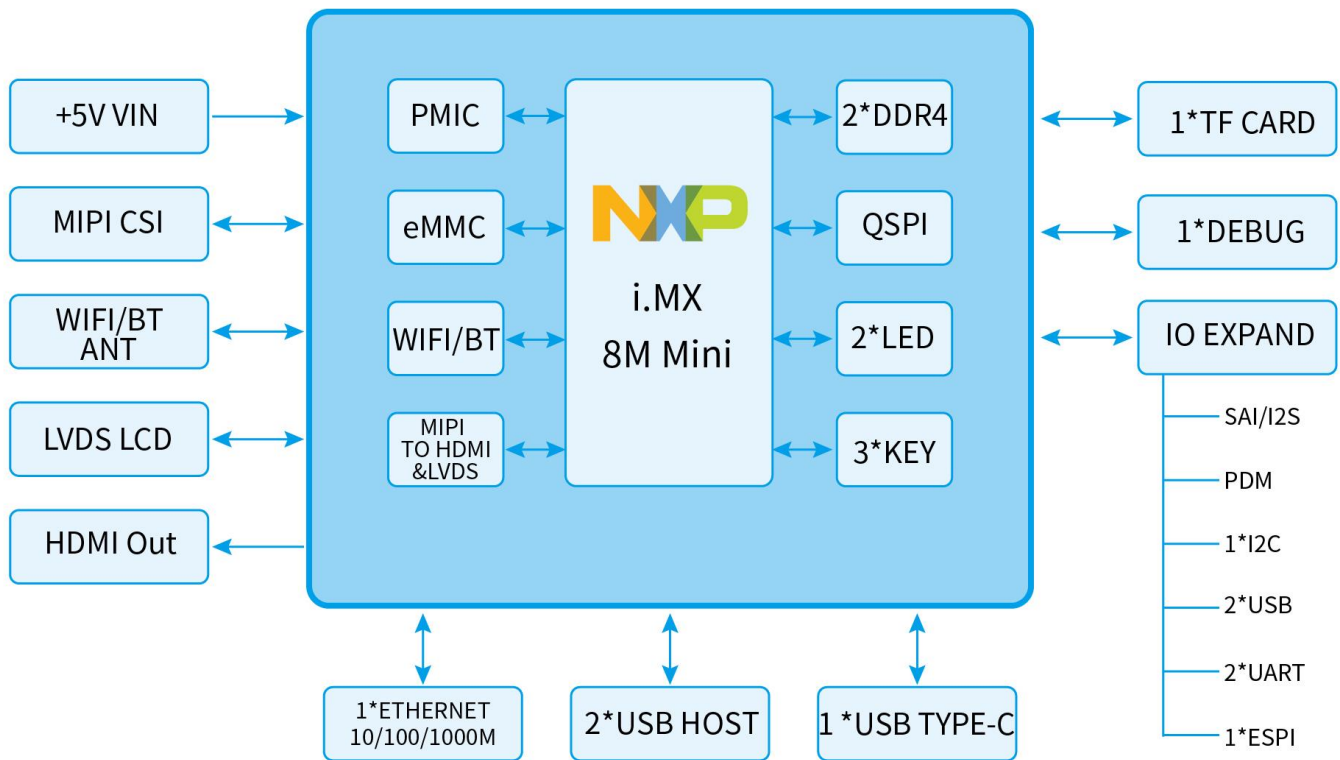
Figure 1-7 MYS-8MMX Function Block Diagram
