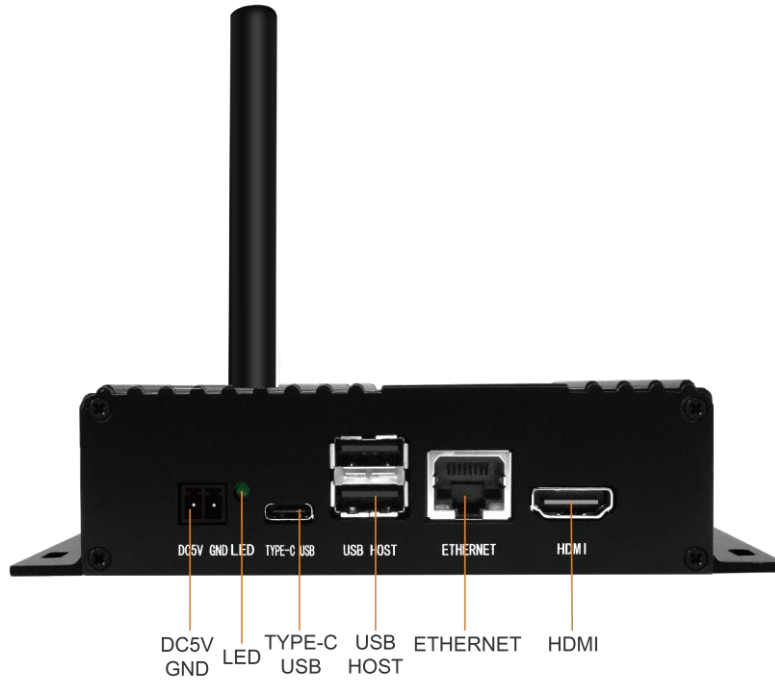
Figure 1-4 MYS-8MMX Box Front-View
