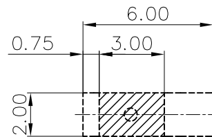
SOLDER PAD DIMENSION
