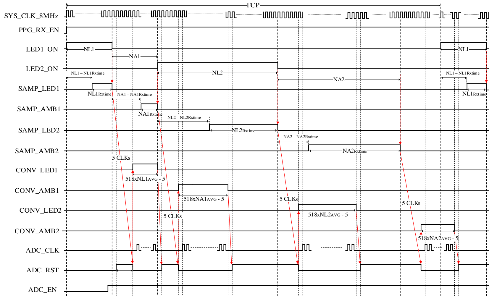
Figure 11 NNC-EPC001 PPG Timing Diagram
