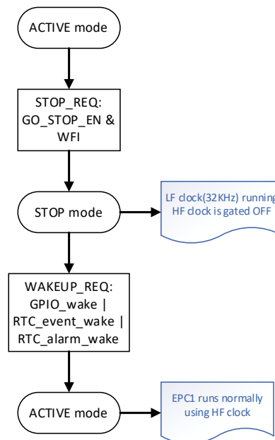
Figure 6 NNC-EPC001 Power-saving mode transition
