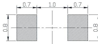
推荐焊盘尺寸 Recommended Soldering Pad
