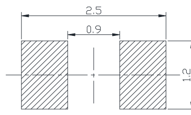
推荐焊盘尺寸 Recommended Soldering Pad
