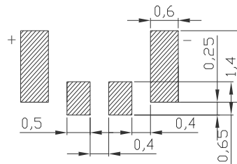
推荐焊盘尺寸 Recommended Soldering Pad
