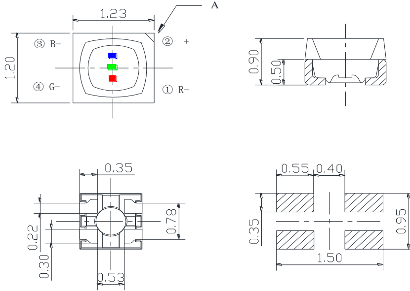
参考焊盘 Reference Soldering Pad
