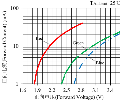
Volt-Ampere Characteristics
