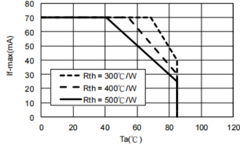
Fig.6- Maximum Driving Forward DC Current vs. Ambient Temperature(Derating based on Tj max=110°C)
