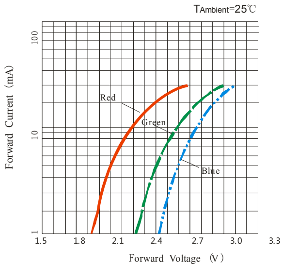
Volt-Ampere Characteristics
