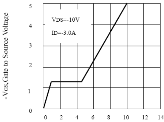
Figure9. Gate Charge
