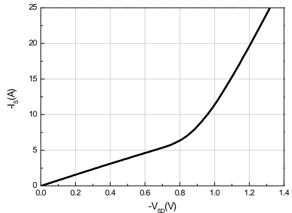
Fig 6: Body-Diode Characteristics
