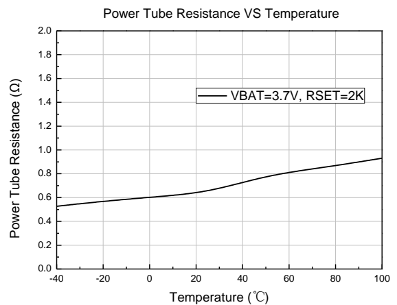
18. Power Tube Resistance VS Temperature
