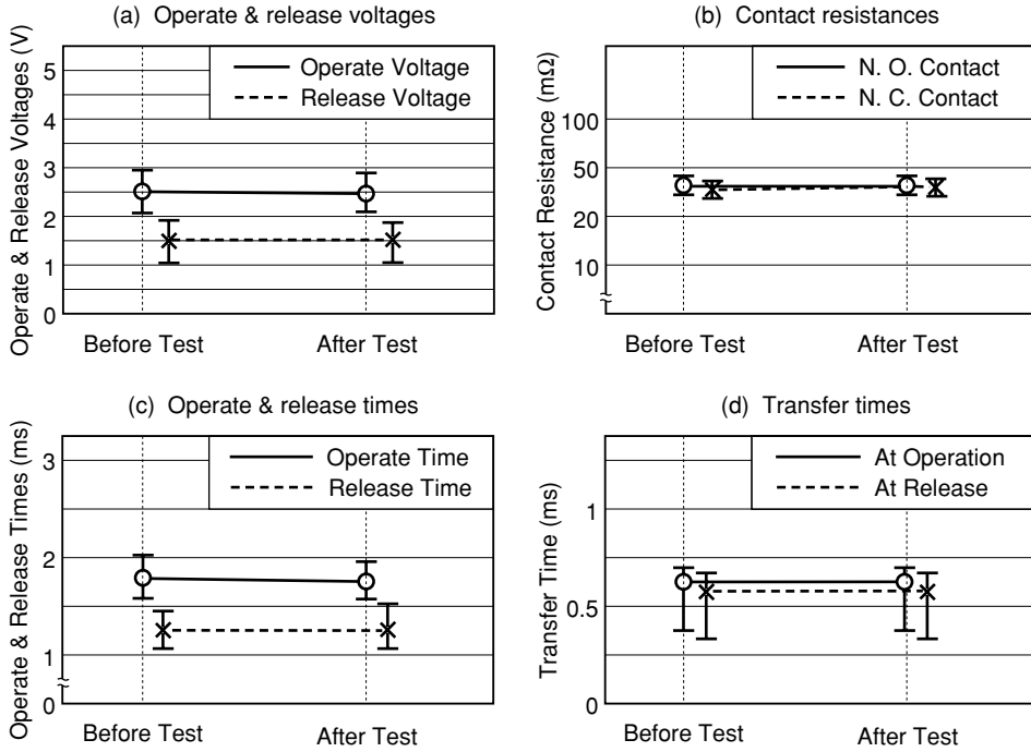
Figure 5.8 (1) Terminal Strength
