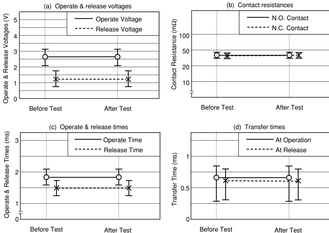
Figure 5.1 (1) High-temperature Test
