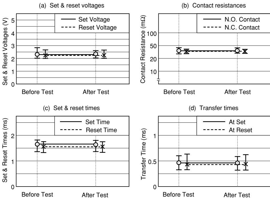
Figure 5.8 (2) Terminal Strength
