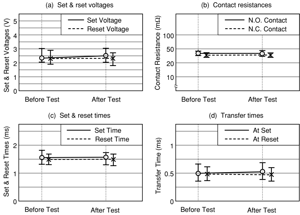
Figure 5.5 (2) Vibration Test
