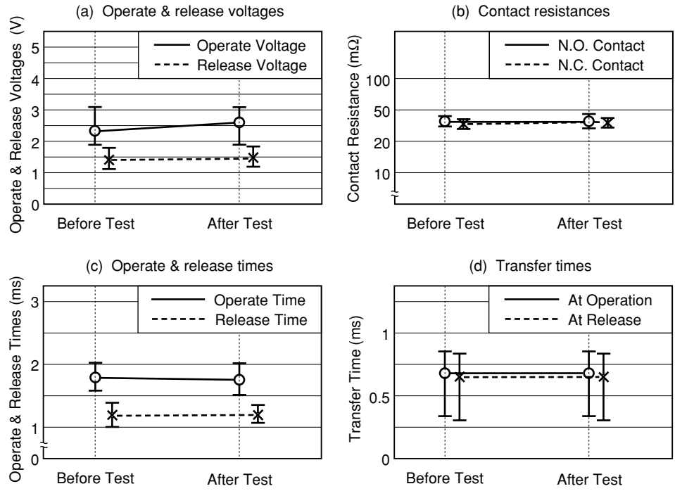
Figure 5.5 (1) Vibration Test
