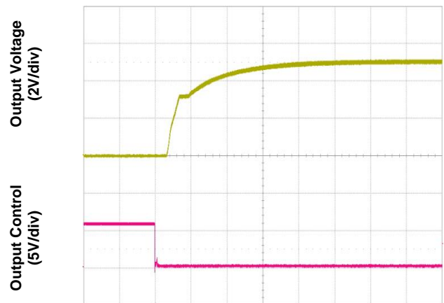
Figure 6. Start-Up from Enable Control
