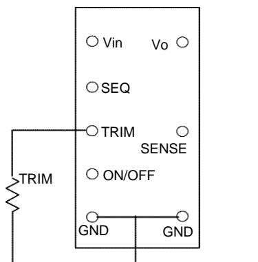
Fig. 15 Circuit to Trim Output Voltage.
