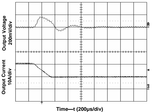
Figure 8. Transient Load Response Input voltage 12V, Output current 20A->10A, Slew rate 0.5A/ \mu s.
