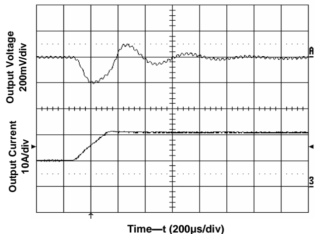
Figure 9. Transient Load Response Input voltage 12V, Output current 10A -> 20A, Slew rate 0.5A/ \mu s
