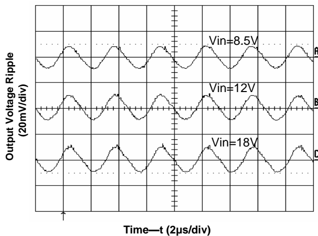
Figure 2. Output Ripple Voltage at 2.5V, 20A Output
