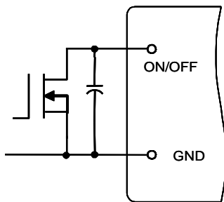
Fig. 13 Circuit for Positive Logic Control
