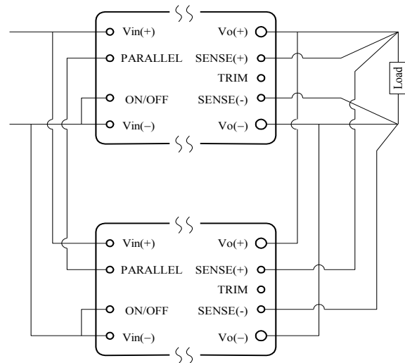
Fig. 20 Circuit Configuration for Active Current Share
