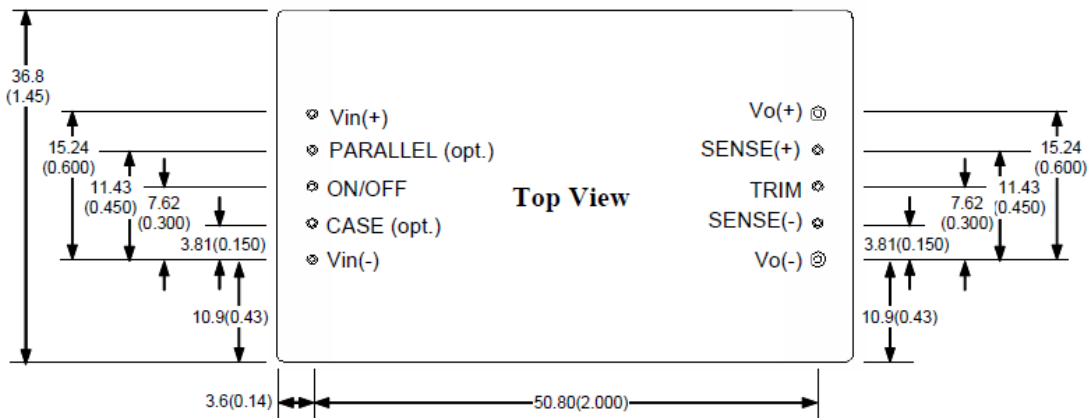
Figure 22. Open frame converter
