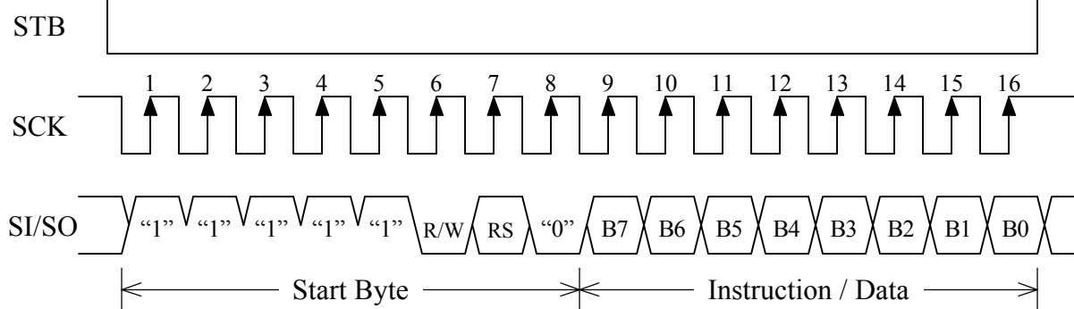
Fig. 10. Typical Synchronous Serial Interface Write Cycle
