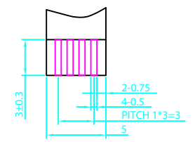
FPC DETAIL(1:3)
