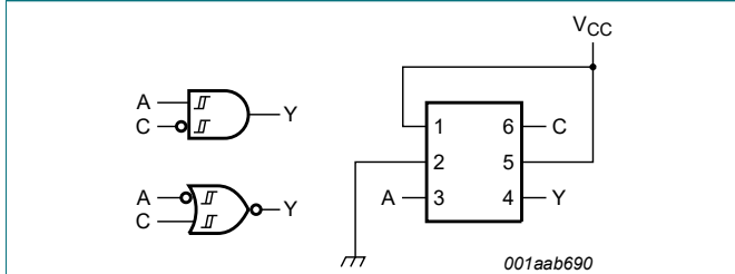
Fig. 7. 2-input AND gate with inverted C input or 2-input NOR gate with inverted A input
