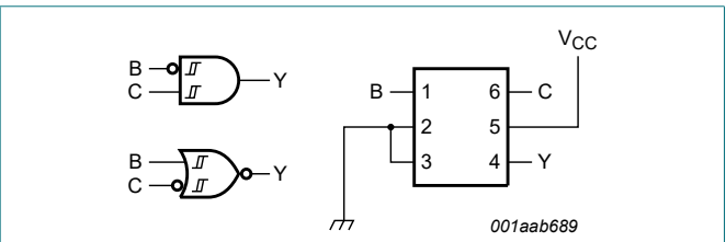
Fig. 6. 2-input AND gate with inverted B input or 2-input NOR gate with inverted C input
