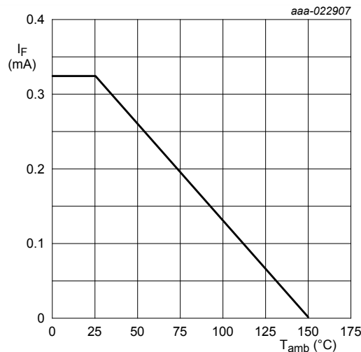
Fig. 1. Forward current as a function of ambient temperature; derating curve
