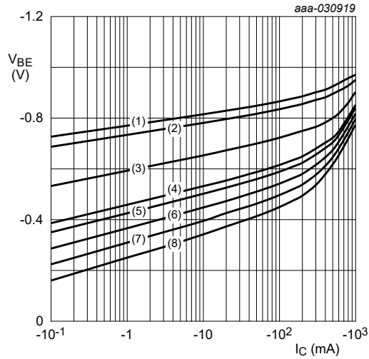
V_{CE} = -5\text{ V} (1) T_{amb} = -55\text{ }^{\circ}\text{C} (2) T_{amb} = -40\text{ }^{\circ}\text{C} (3) T_{amb} = 25\text{ }^{\circ}\text{C} (4) T_{amb} = 85\text{ }^{\circ}\text{C} (5) T_{amb} = 100\text{ }^{\circ}\text{C} (6) T_{amb} = 125\text{ }^{\circ}\text{C} (7) T_{amb} = 150\text{ }^{\circ}\text{C} (8) T_{amb} = 175\text{ }^{\circ}\text{C}
