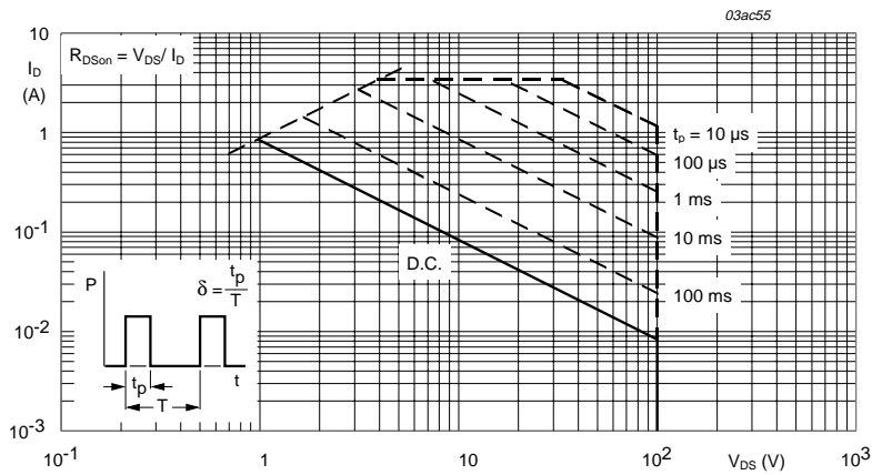
Fig 3. Safe operating area; drain and peak currents as a function of drain source voltage.
