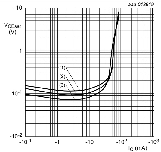
Fig. 9. Collector-emitter saturation voltage as a function of collector current; typical values I_C/I_B = 5 (1) T_{amb} = 100\text{ °C} (2) T_{amb} = 25\text{ °C} (3) T_{amb} = -55\text{ °C}
