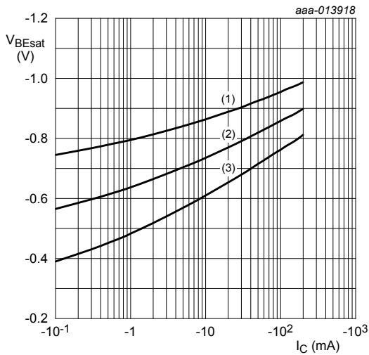
Fig. 8. Base-emitter saturation voltage as a function of collector current; typical values I_C/I_B = 5 (1) T_{amb} = -55\text{ °C} (2) T_{amb} = 25\text{ °C} (3) T_{amb} = 100\text{ °C}
