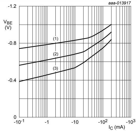
Fig. 7. Base-emitter voltage as a function of collector current; typical values V_{CE} = -10\text{ V} (1) T_{amb} = -55\text{ °C} (2) T_{amb} = 25\text{ °C} (3) T_{amb} = 100\text{ °C}
