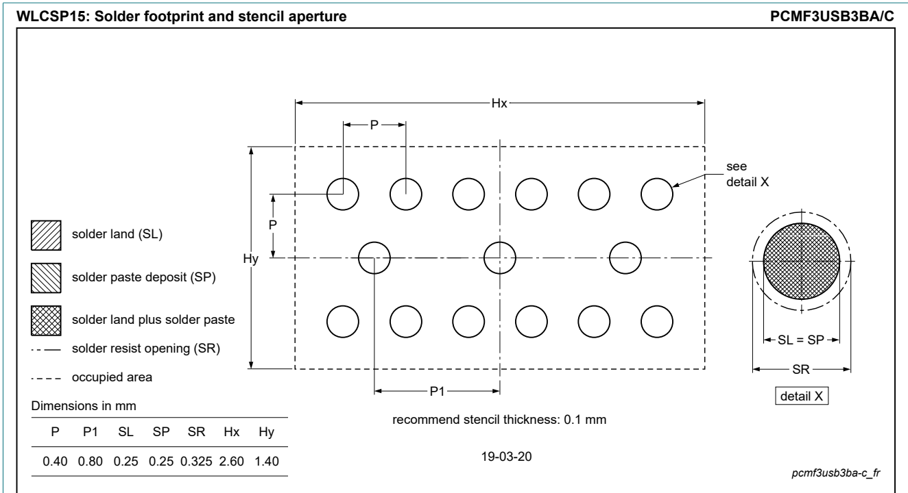
Fig. 25. Soldering footprint WLCSP15 (PCMF3USB3BA/C)
