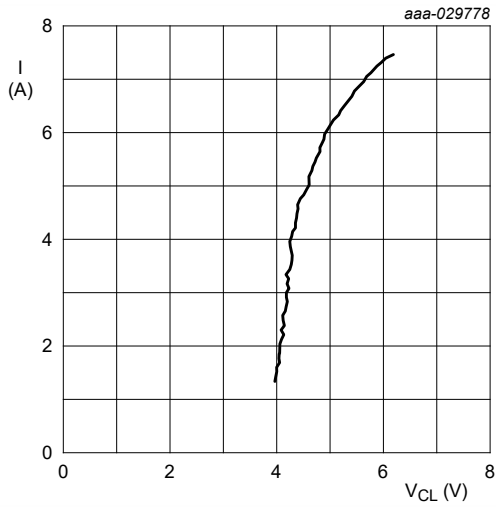
Fig. 17. Dynamic resistance with positive clamping; typical values
