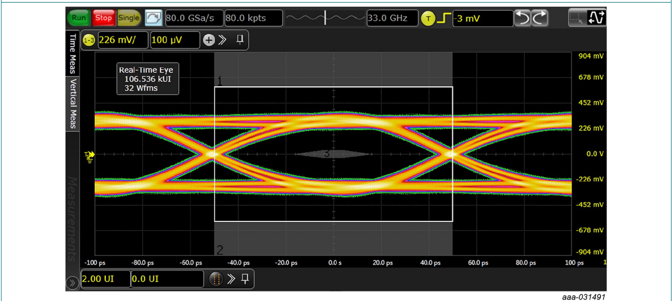
Fig. 6. USB3.2 eye diagram 10 Gbps, PCB without device; typical values
