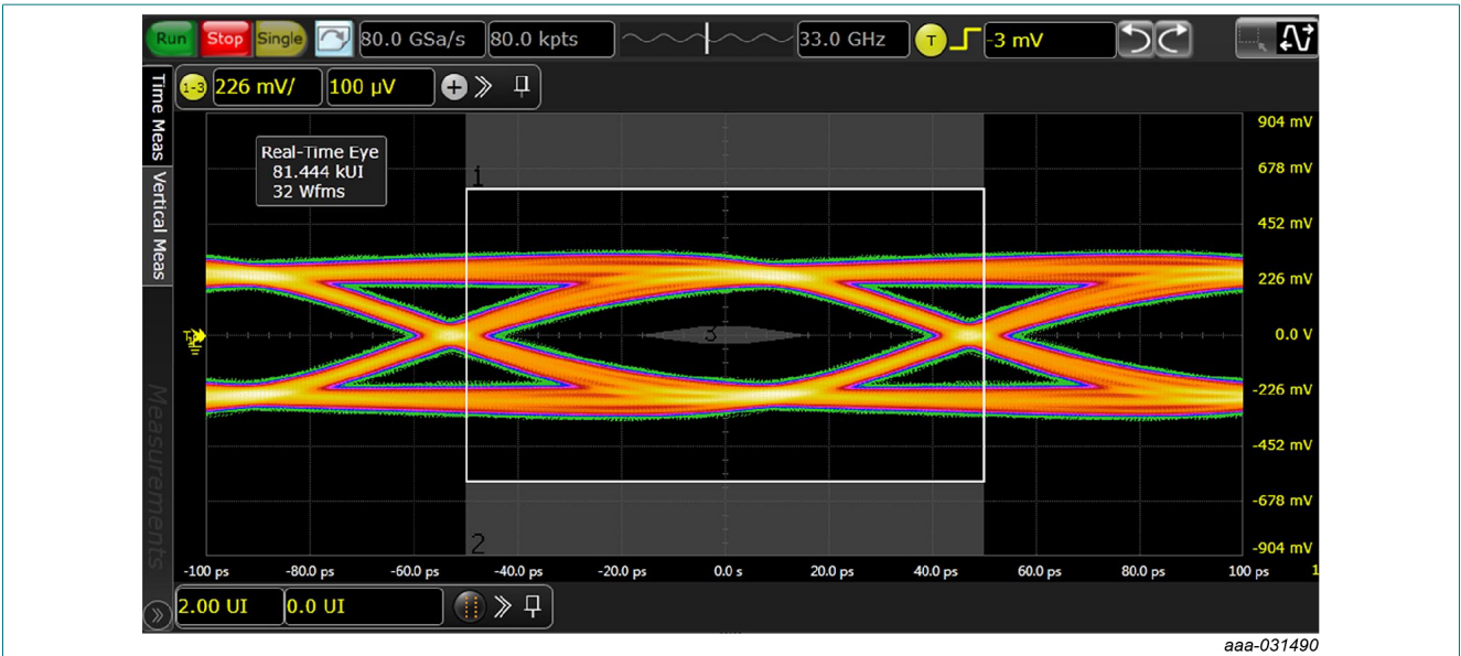
Fig. 5. USB3.2 eye diagram 10 Gbps, PCB with device; typical values
