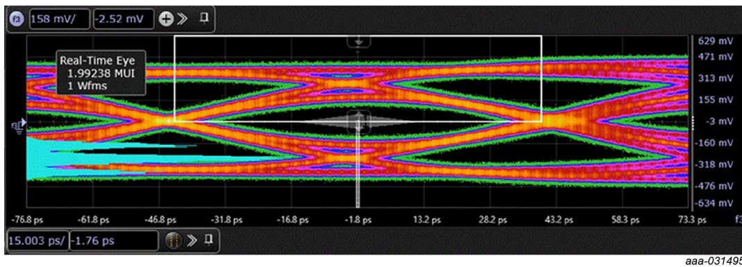
Fig. 9. HDMI 2.1 12G FRL eye diagram, PCB with device; typical values
