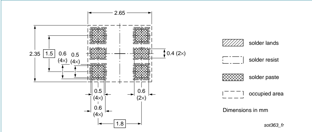
Fig 13. Reflow soldering footprint PUMB10 (SOT363/SC-88)
