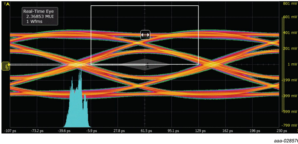
Fig. 11. HDMI 2.0 eye diagram TP2, test board without device; typical values
