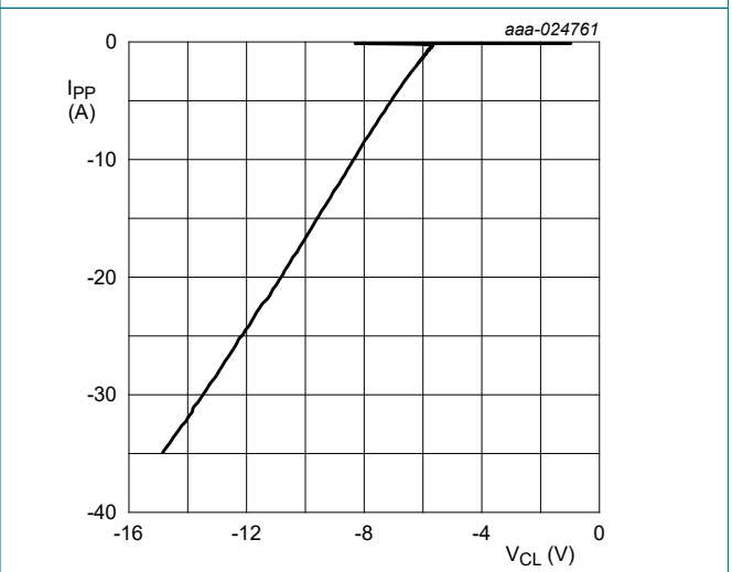
Fig. 6. Negative clamping voltage (TLP); typical values t_p = 100\text{ ns} ; Transmission Line Pulse (TLP)
