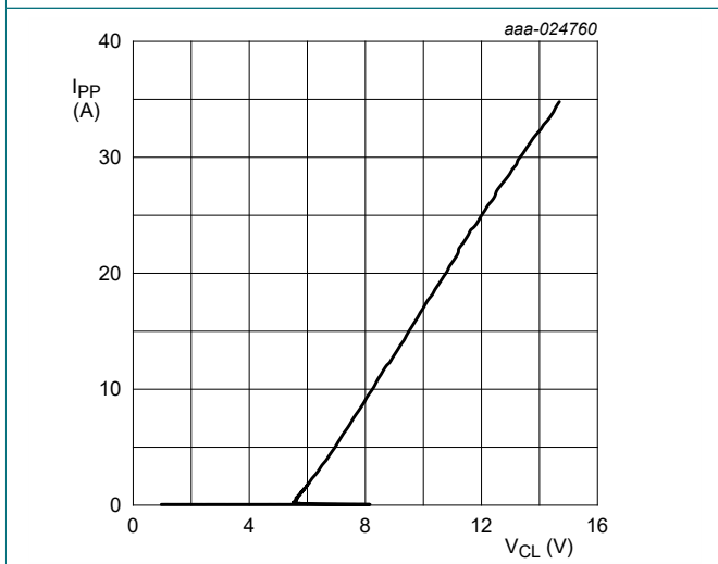
Fig. 5. Positive clamping voltage (TLP); typical values t_p = 100\text{ ns} ; Transmission Line Pulse (TLP)
