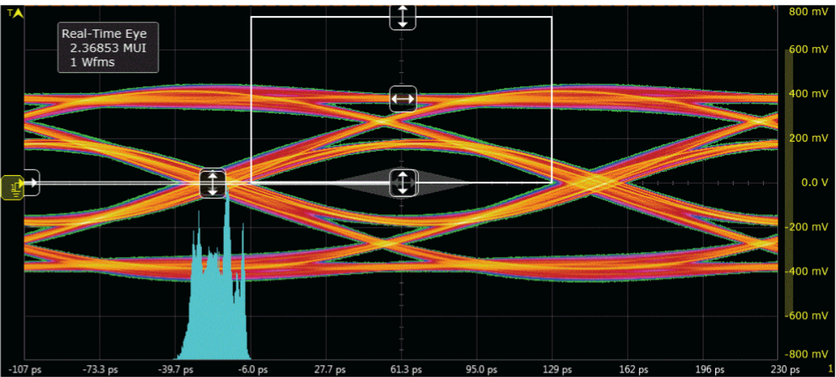
Fig. 12. HDMI2.0 TP2 eye diagram, PCB with device; typical values
