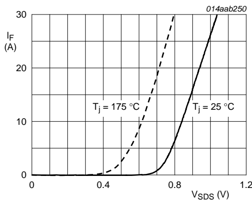
Fig 14. Source (diode forward) current as a function of source-drain (diode forward) voltage; typical values
