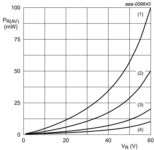
T_j = 150\text{ °C} (1) \delta = 1 (2) \delta = 0.5 (3) \delta = 0.2 (4) \delta = 0.1
