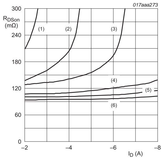
Fig 8. Drain-source on-state resistance as a function of drain current; typical values T_j = 25\text{ °C} (1) V_{GS} = -2.0\text{ V} (2) V_{GS} = -2.25\text{ V} (3) V_{GS} = -2.5\text{ V} (4) V_{GS} = -3.0\text{ V} (5) V_{GS} = -3.5\text{ V} (6) V_{GS} = -4.5\text{ V}
