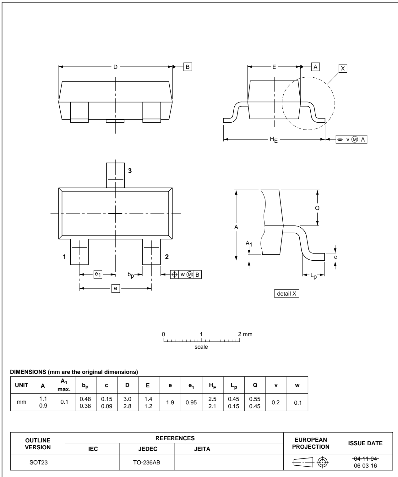
Fig 17. Package outline SOT23 (TO-236AB)
