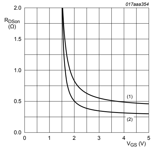
(1) T_j = 150\text{ }^\circ\text{C} (2) T_j = 25\text{ }^\circ\text{C} Fig. 9. Drain-source on-state resistance as a function of gate-source voltage; typical values
