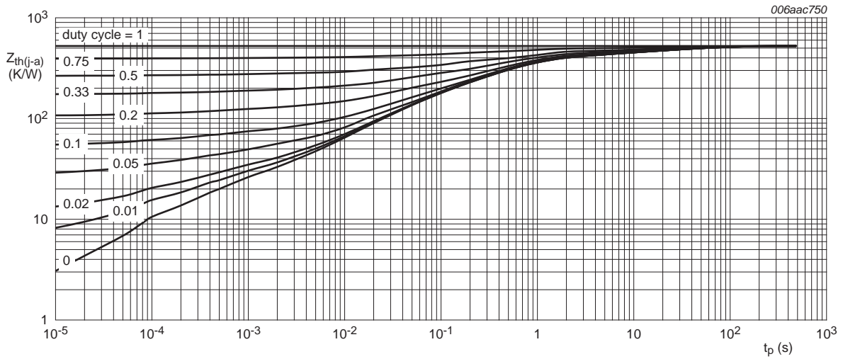
Fig 3. Per transistor: Transient thermal impedance from junction to ambient as a function of pulse duration for PUMB9 (SOT363); typical values
