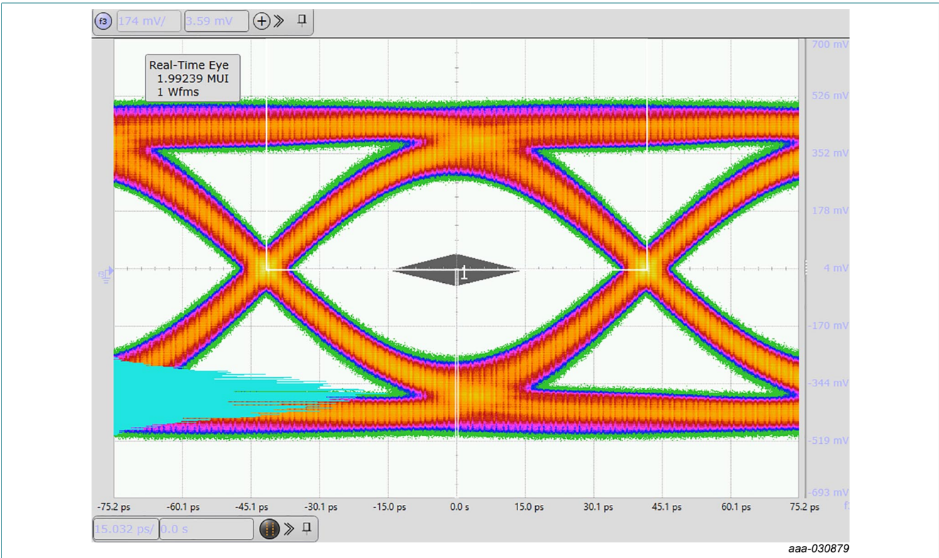
Fig. 8. HDMI 2.1 12G FRL TP1 eye diagram, PCB with device; typical values
