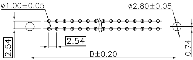
PCB LAYOUT
