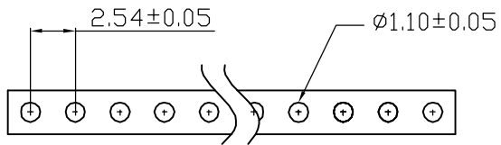
PCB LAYOUT
