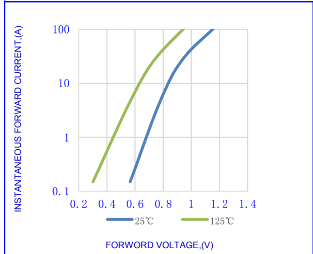
Fig.2-TYPICAL INSTANTANEOUS FORWARD
